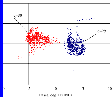
Figure 7: Phase space plots of a two-charge state beam just prior to the first stripper.
